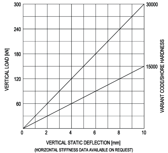
LOAD CHARACTERISTICS
