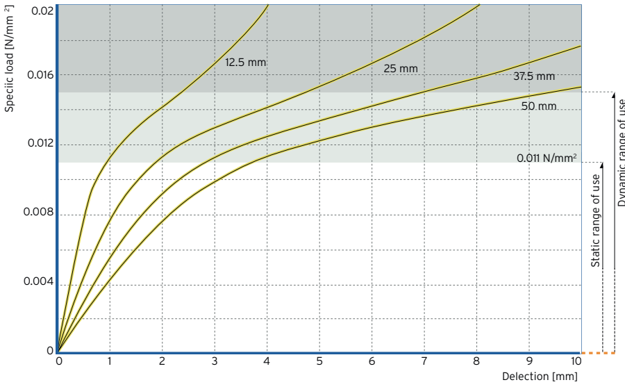
Figure 1: Quasistatic load delection curve measured with a loading rate of 0.0011 N/mm 2 /s
