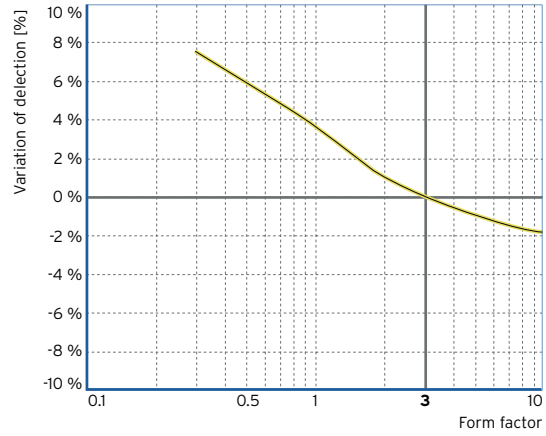
Figure 6: Delection*
