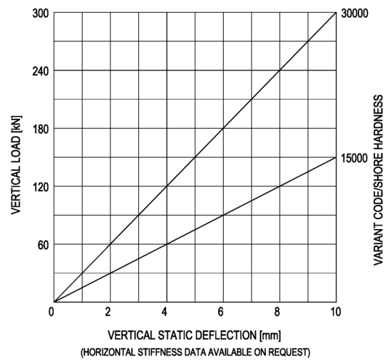
LOAD CHARACTERISTICS
